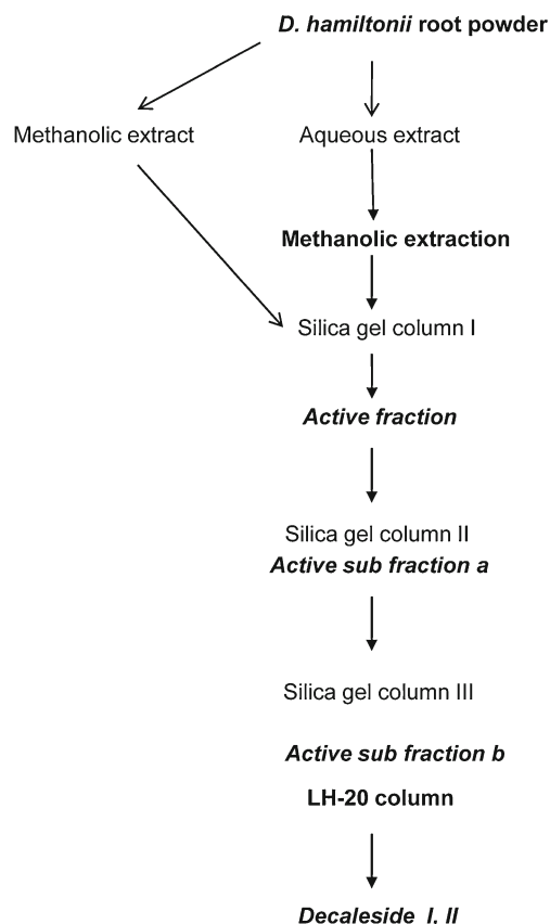
Fig. 1 Scheme for the isolation of the Decalesides I and II from the methanolic and aqueous extracts of the roots of D. hamiltonii
