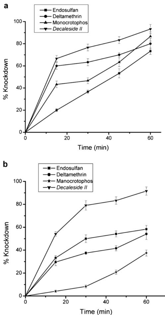
Fig. 3 Comparison of the insecticidal action (timecourse) of Decaleside II with that of chemical insecticides in a Musca domestica (housefly) and b Blatella germanica exposure at LC 50 by contact bioassay ( n=4 , error bars, SEM)
