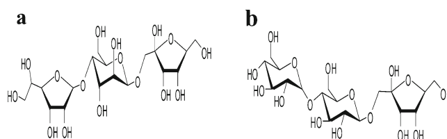
Fig. 2 Molecular structures: a Decaleside I (α-D-Gulosefuranose-(1-4)-β-D-altrosepyranosyl-(1-1)-α-D-psicosefuranose); b Decaleside II (β-D-Galactopyranose-(1-4)-α-D-altrosepyranosyl-(1-1)-α-D-psicosefuranose)
