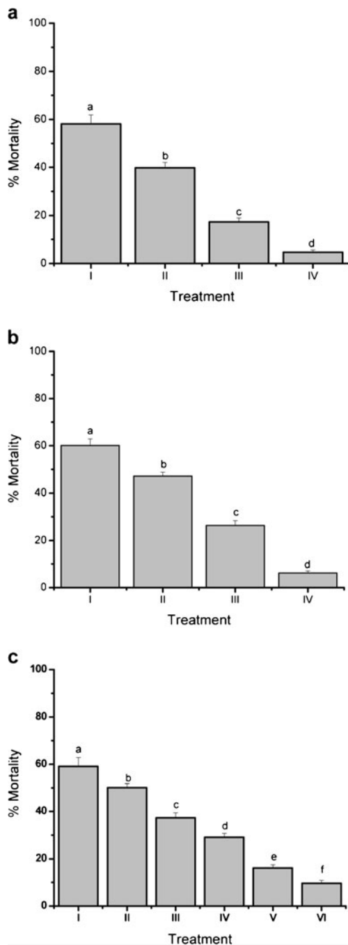
Fig. 5 Effect of sugars on the insecticidal activity of Decaleside II in German cockroach exposure at LC_{50} ( 0.07 \text{ mg/cm}^2 ) by contact bioassay. a Monosaccharide (glucose). I Decaleside II , II Decaleside II + glucose (1:1), III Decaleside II + glucose (1:2), IV Decaleside II + glucose (1:3). Ratio in molar concentration ( n=4 , error bars, SEM), one-way ANOVA, P<0.001 . b Disaccharide (trehalose). I Decaleside II , II Decaleside II + trehalose (1:1), III Decaleside II + trehalose (1:2), IV Decaleside II + trehalose (1:3). Ratio in molar concentration ( n=4 , error bars, SEM), one-way ANOVA, P<0.001 . c Trisaccharide (maltotriose). I Decaleside II , II Decaleside II + maltotriose (1:0.1), III Decaleside II + maltotriose (1:0.25), IV Decaleside II + maltotriose (1:0.5), V Decaleside II + maltotriose (1:0.75), VI Decaleside II + maltotriose (1:1). Ratio in molar concentration ( n=4 , error bars, SEM), one-way ANOVA, P<0.001
