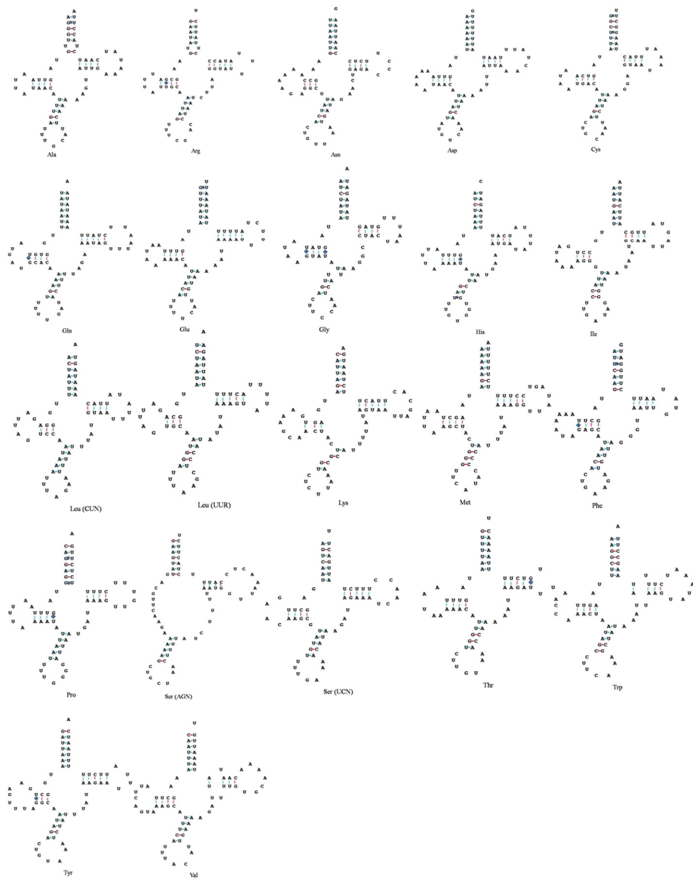
Fig. 3. Predicted secondary clover-leaf structures for the 22 tRNA genes of B. zonata . The tRNAs are labeled with abbreviation of their corresponding amino acids below each tRNA gene structure. Arms of tRNAs (clockwise from top) are the amino acid acceptor arm, TYC arm, the anticodon arm, and dihydrouridine (DHU) arm.
